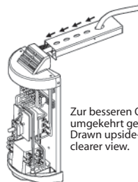
Abb.4 | Fig.4 Kabelverbindung Cable Connection
